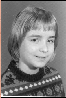
B21-ph6
